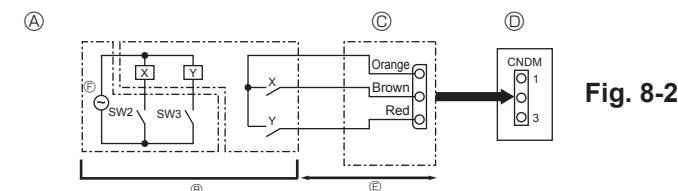
Fig. 8-2 ① Circuit diagram example (Demand function) ② On-site arrangement X, Y: Relay ③ External input adapter (PAC-SC36NA-E) ④ Outdoor unit control board ⑤ Max. 10 m ⑥ Power supply for relay
